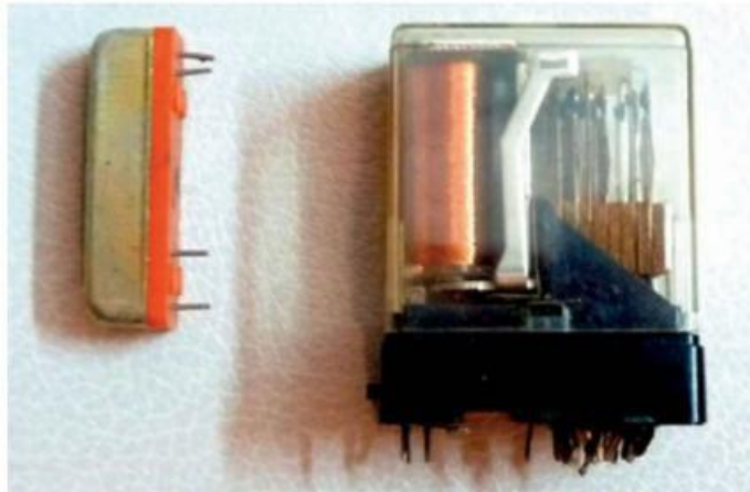
Figure 9-38. Relais standards
