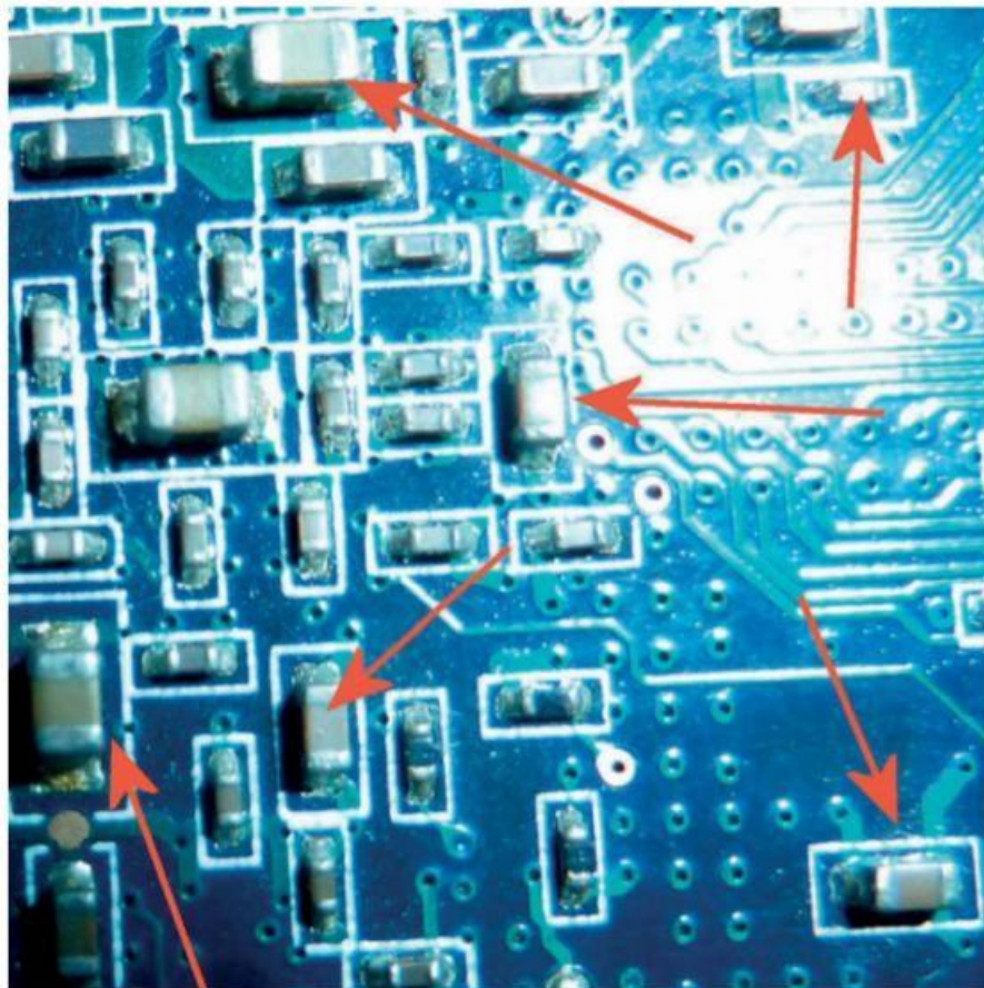
Figure 9-13. Condensateurs CMS non polarisés
