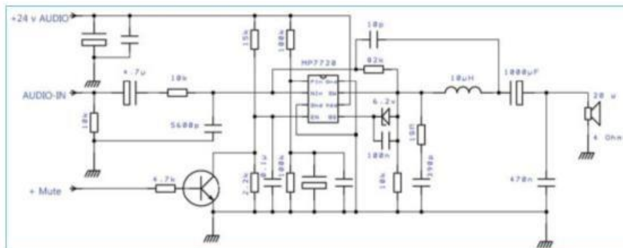
Figure 4-38. Amplificateur monophonique classe D 20 W (circuit MP7720)
