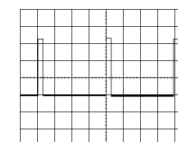
⑤ (IC301-67) 4.6Vp-p 2V/10usec/cm PICTURE SEARCH
