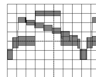
③ (IC301-43) 520mVp-p 100mV/5usec/cm PLAY
