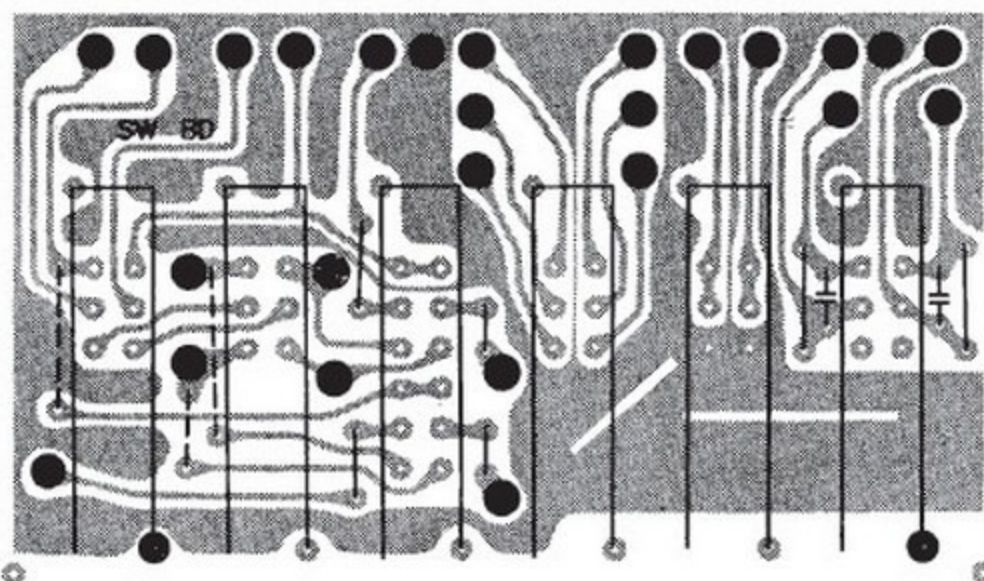
A437/A457 SWITCH BOARD Assy No. 100-1352-044
