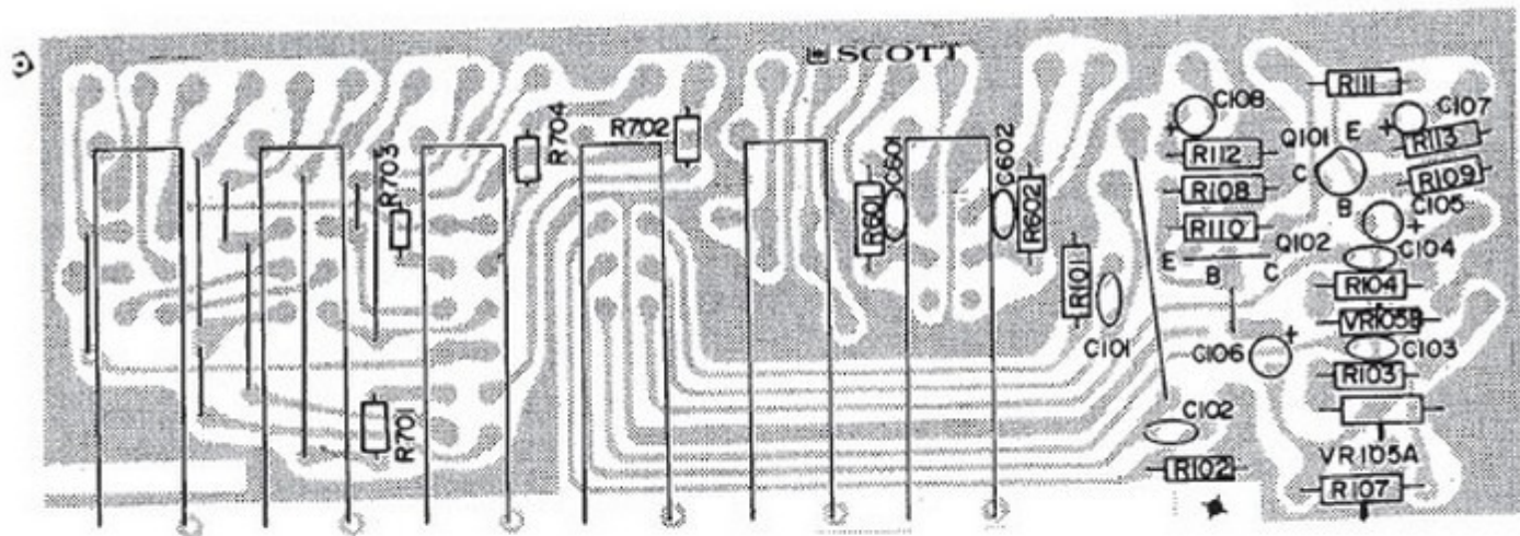
A437 TONE BOARD "B" Assy No. 100-1334-046
