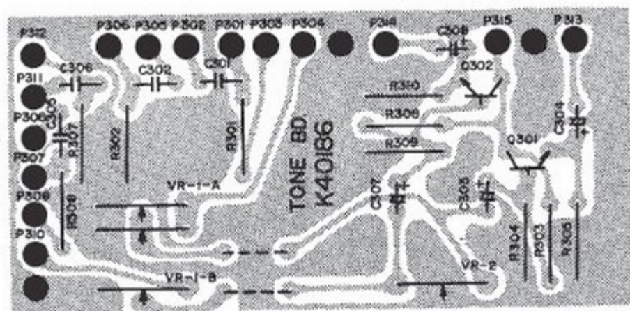
A 457 TONE BOARD "A" Assy No. 100-1334-042
