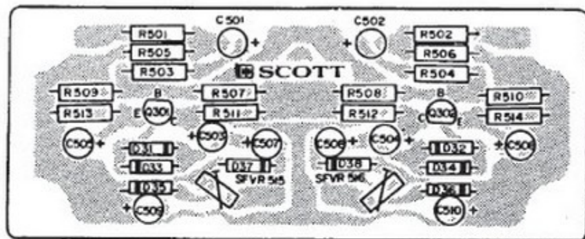
A437 METER DRIVE Assy No. 100-1335-032
