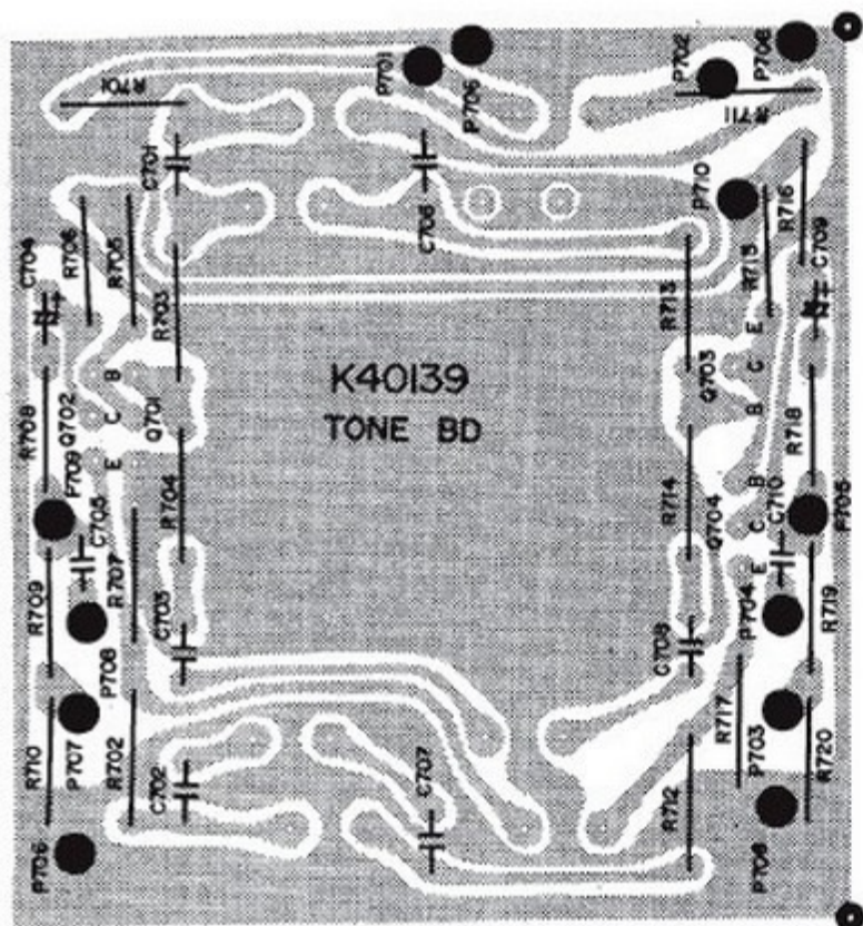
A437 TONE BOARD "B" Assy No. 100-1334-048
