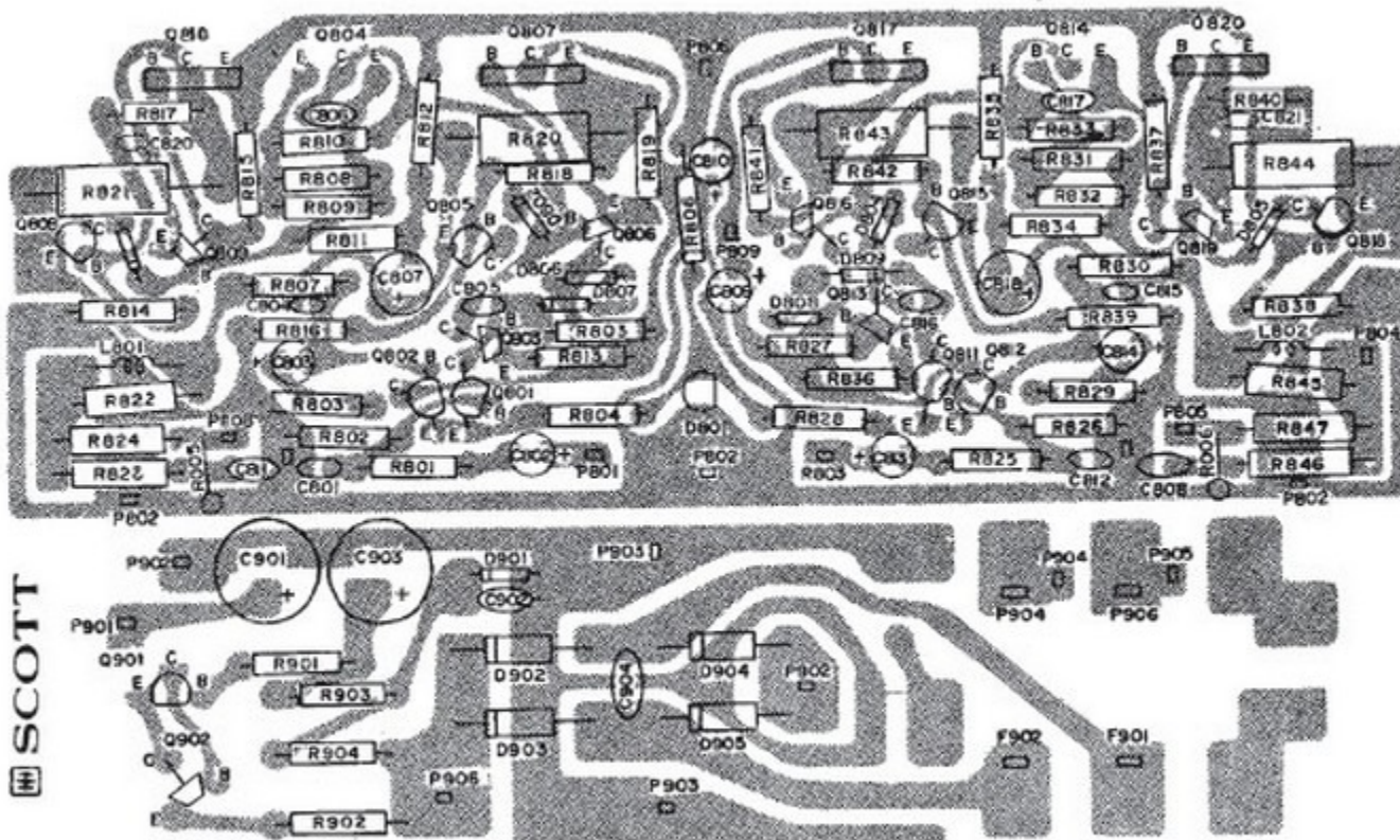
A417 DRIVER/REGULATOR Assy No. 100-1335-031
