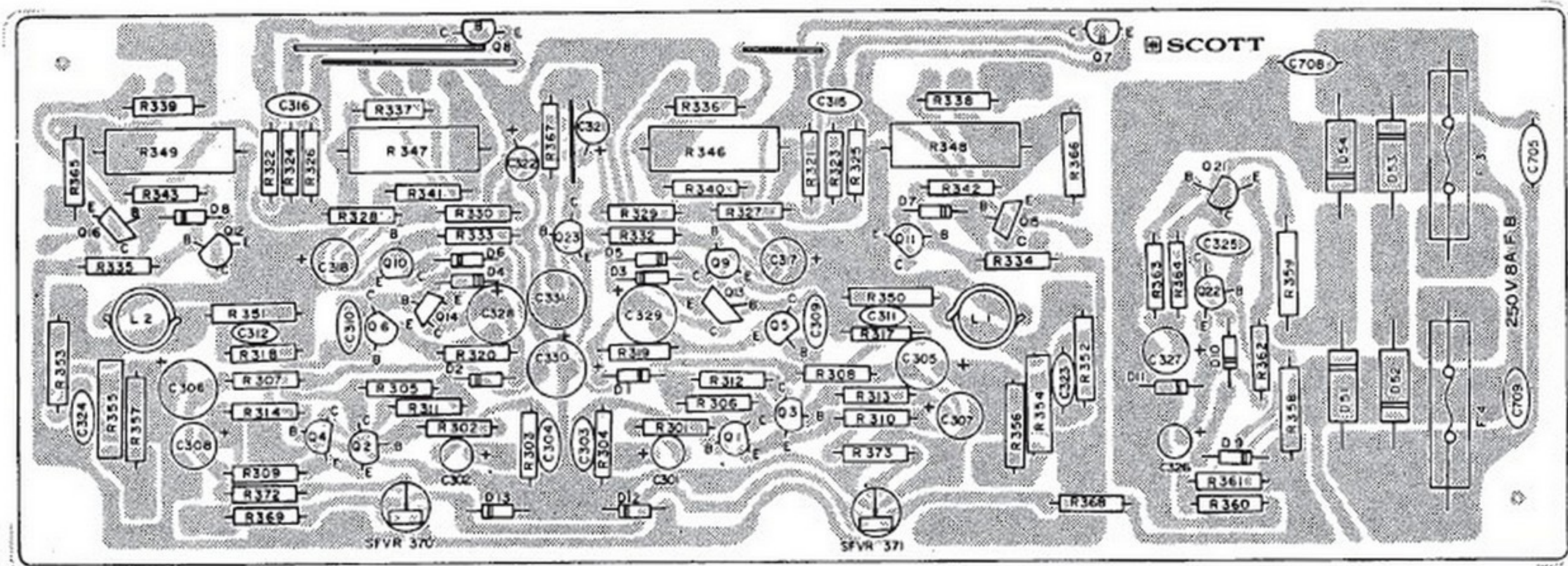
A437 DRIVER/REGULATOR BOARD Assy No. 100-1335-034
