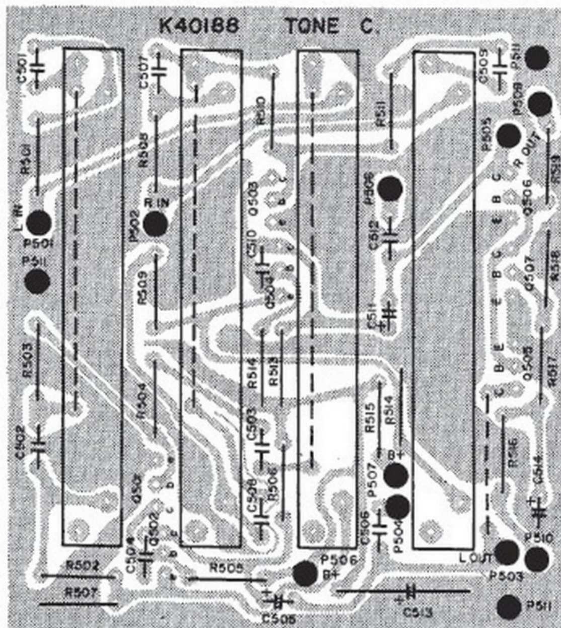
A457 TONE BOARD "C" Assy No. 100-1334-044
