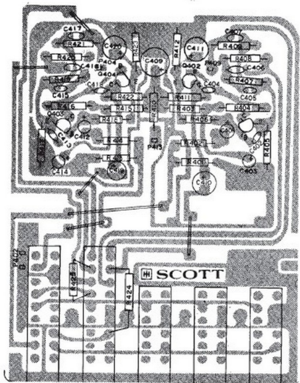
A417 PREAMP SWITCH BOARD Assy No. 100-1333-047
