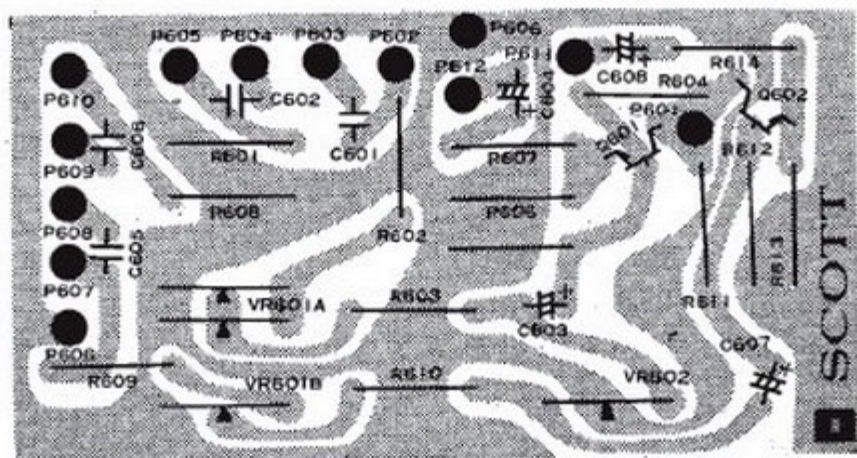
A437 TONE BOARD "A" Assy No. 100-1334-047
