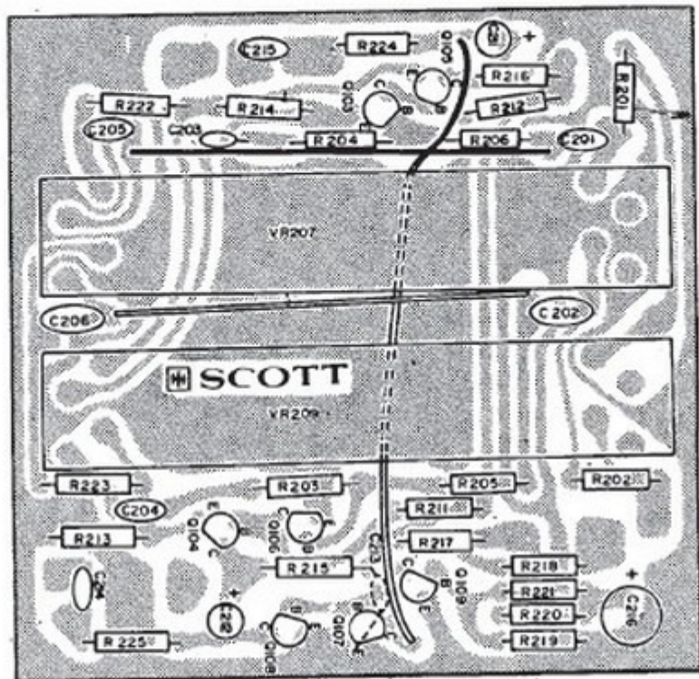
A437 TONE BOARD "A" Assy No. 100-1334-045
