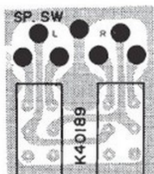
A457 SPEAKER SWITCH BOARD Assy No. 100-1352-045
