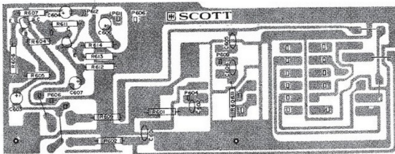
A417 TONE BOARD "B" Assy No. 100-1334-041
