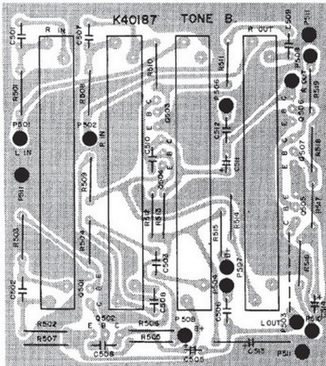
A457 TONE BOARD "B" Assy No. 100-1334-043
