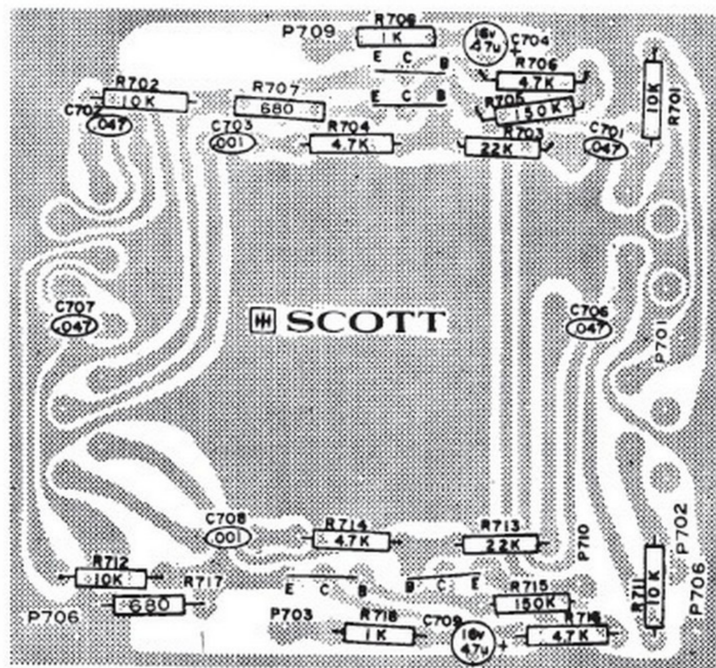
A417 TONE BOARD "A" Assy No. 100-1334-033
