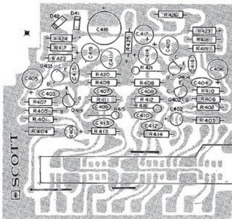
A437 PREAMP/SWITCH BOARD Assy No. 100-1333-048
