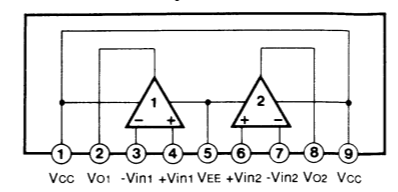
IC704, 707, 711, 712 : \mu PC4570HA Dual OP-Amp
