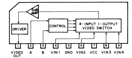
IC855 : LA7956 Video Switch
