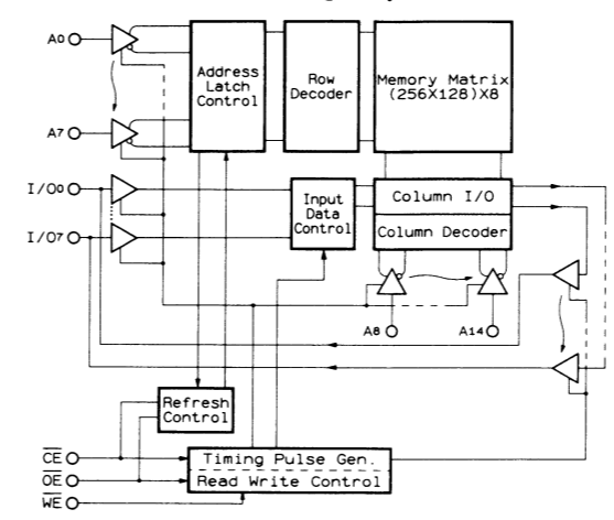
IC702 : HM65256BLSP-10 32768-word x 8-bit High Speed Pseudo Static RAM
