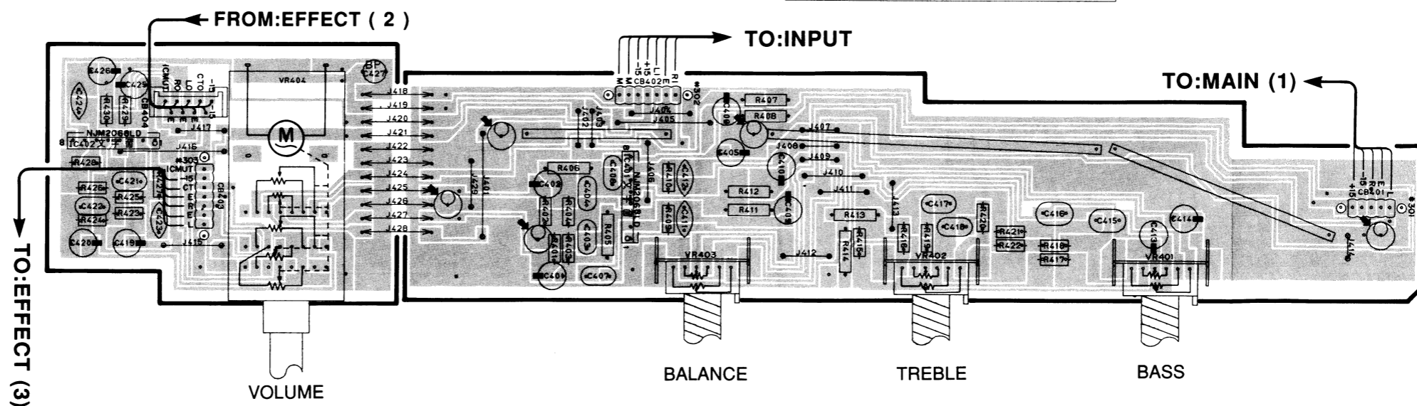
P.C.B. OPERATION ( 2 )
