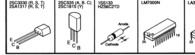
PIN CONNECTION DIAGRAM OF TRANSISTORS, DIODES AND ICs.
