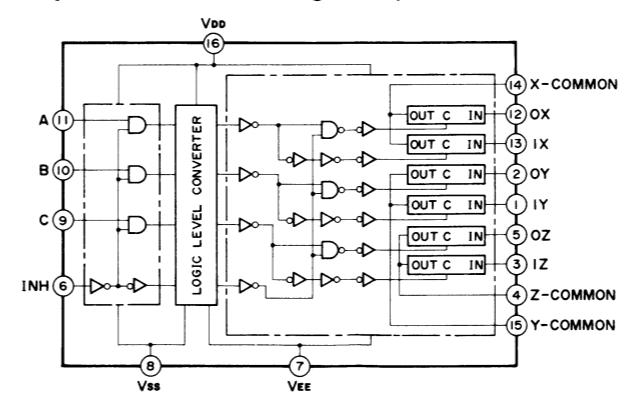
IC713, 714 : TC4053BP Triple 2 Channel Analog Multiplexers/Demultiplexers
