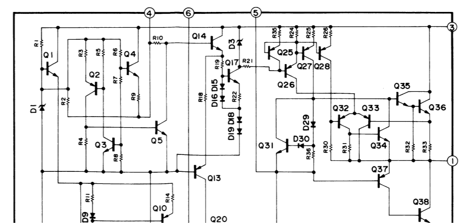
IC802, 803 : \mu PC1188H Power Amp
