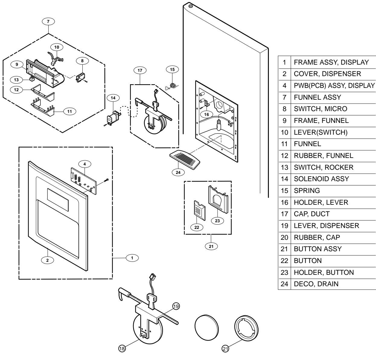
< 17 Cap Assy, Duct Detailed Drawings >
