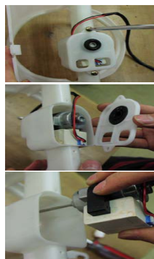
Loosen screws of a motor cover and separate cover and pull out C-fan motor.
