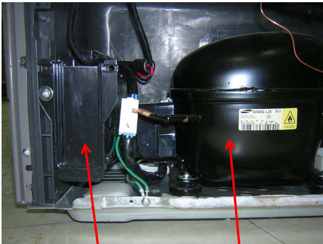
INVERTER BOX
