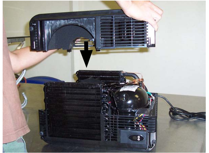
⑧ Put back top.
