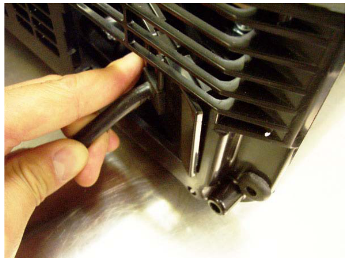
⑥ Insert whole plate assembly into unit and angle right edge out over opening.
