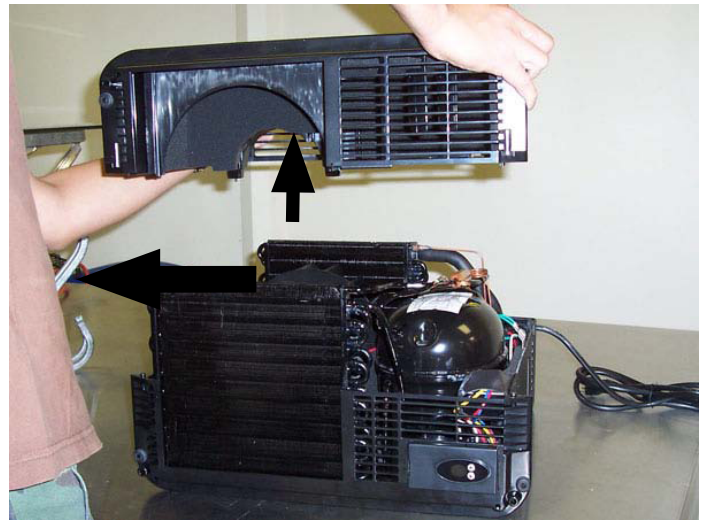
② Lift off top.
