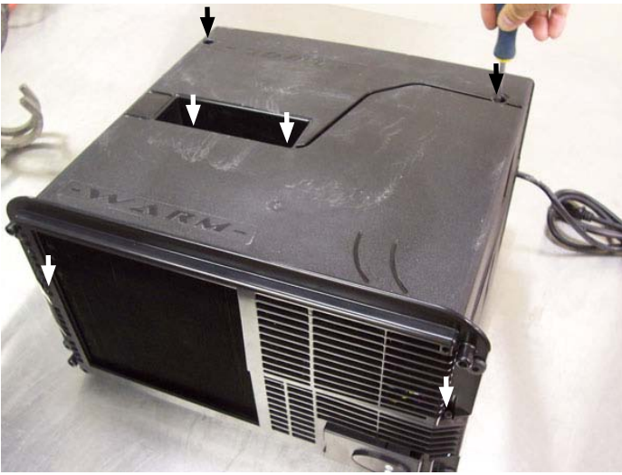
⑨ Screw in all 6 screws.
