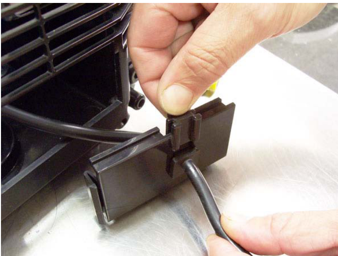
⑤ Slide plate insert down over top of cord.
