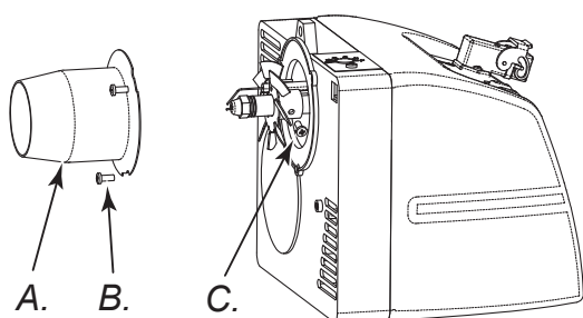
Figure 12 - Disassembly shell-burner
