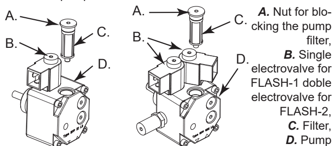
Figur 11 - Pomp of burner
