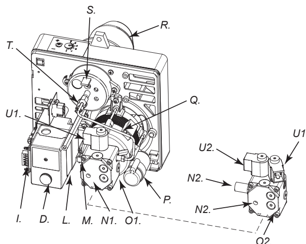
Figur 6 - Components burner
