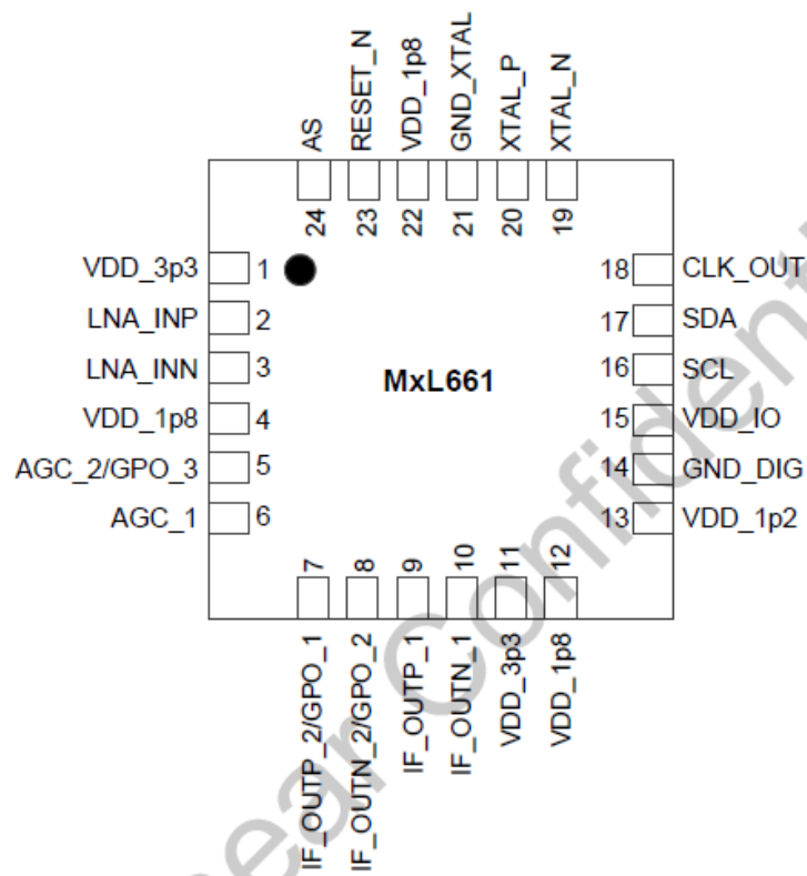
Figure 1 Pin description
