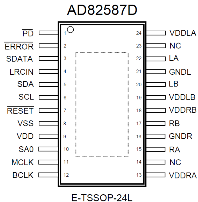
Figure 4 Pin description
