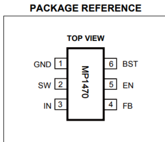
Figure 13 Pin Description
