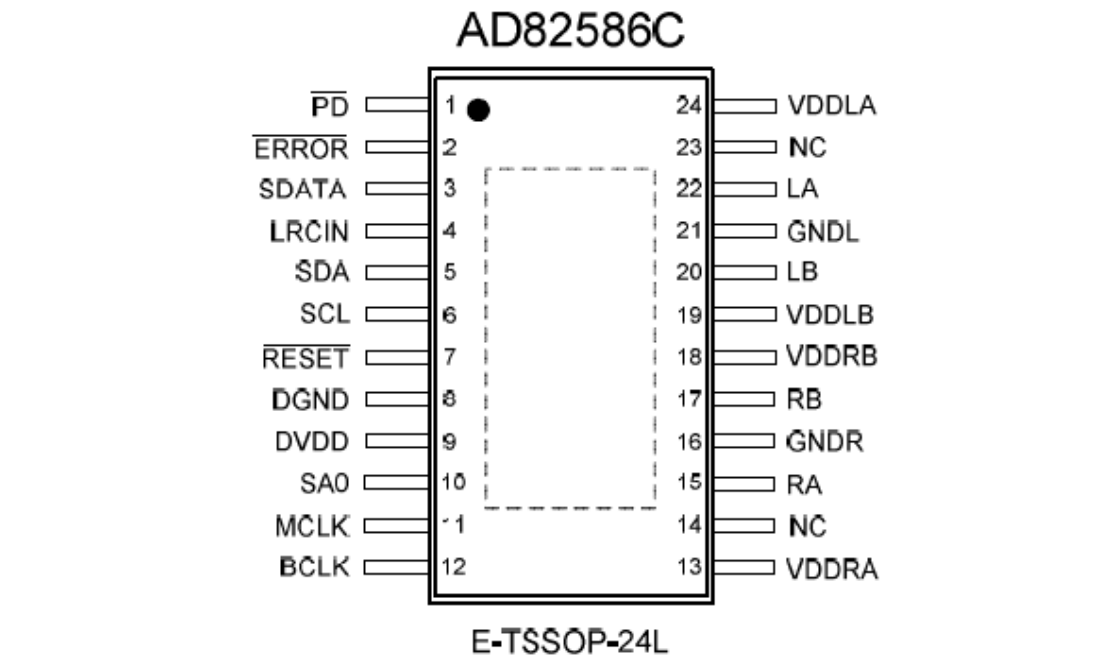
Figure 6 Pin Description
