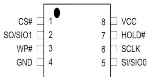
Figure 16 Pin configuration
