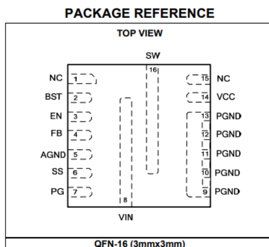
Figure 14 Pin Descriptions
