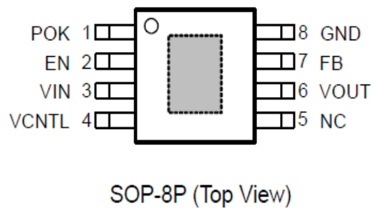
Figure 15 Pin Description
