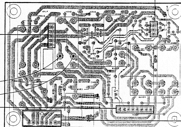
RELAY assembly
