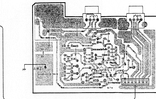
MIC assembly
