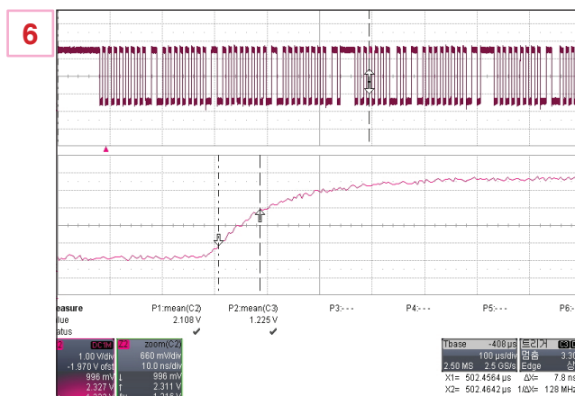
IC202 SCL
