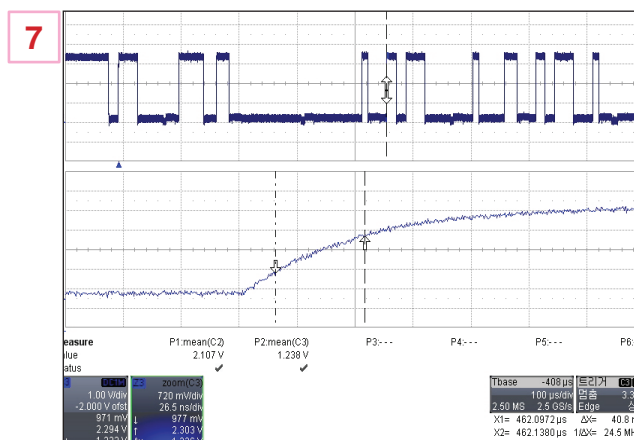
IC202 SDA
