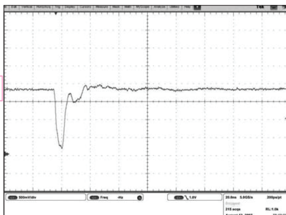
IC501 MT8563 WE#
