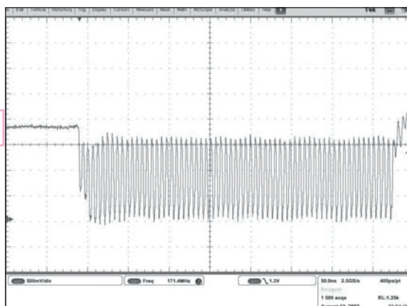
IC501 MT8563 CAS#
