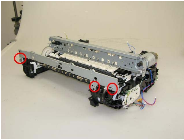
Remove the front chassis (3 screws).
