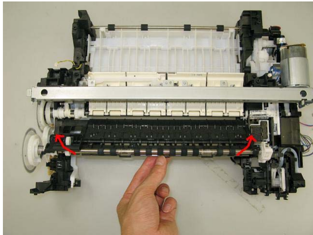
While raising the front of the platen unit, remove the platen unit from the printer unit.
