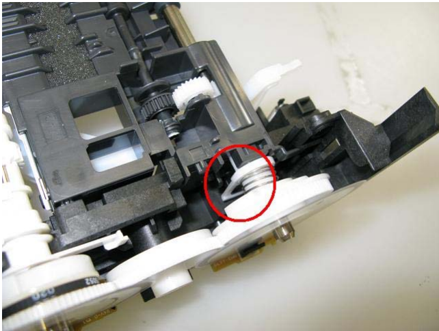
Unlock the paper eject roller gear.
